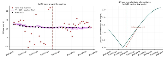
Fig. 2. Sensitivity of day length to latitude through the deployment. The derivative passes through zero at the March equinox, where latitude is unobservable from day length at any noise level.
